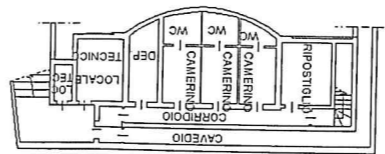
PIANO INTERRATO H=2.70
